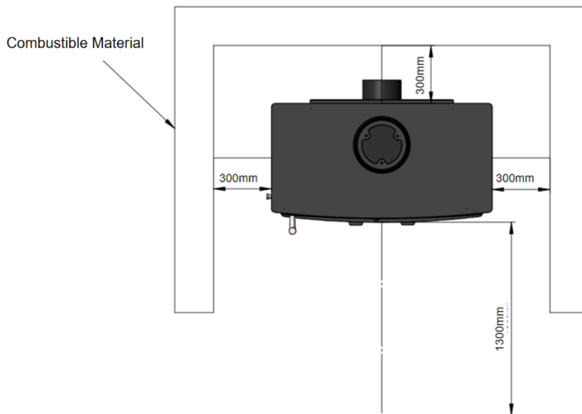
The distance to combustibles of Chadwick 8
