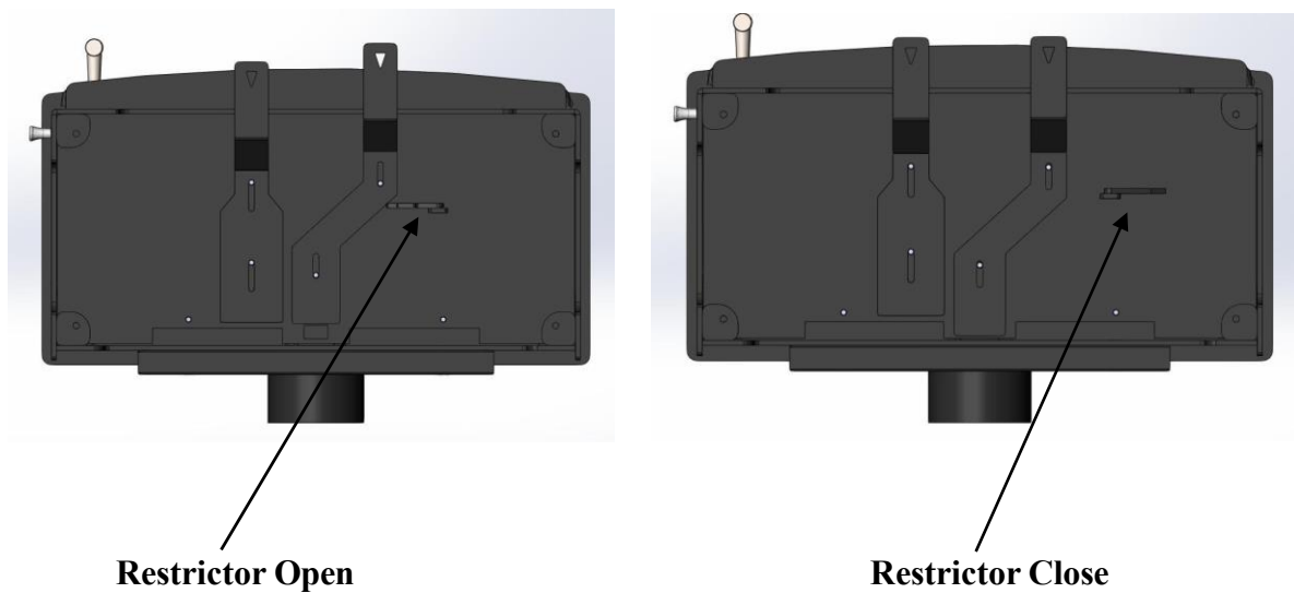
Fig. 3. Fitted Smoke Exemption Restrictor
