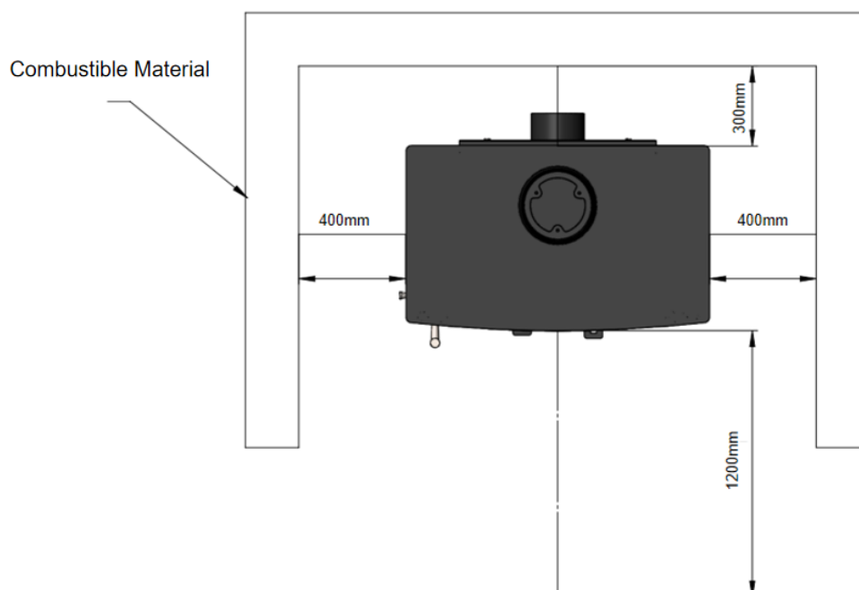
The distance to combustibles of Chadwick 12
