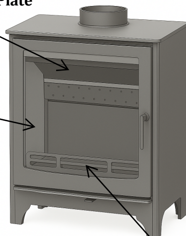
Fuel Retainer
